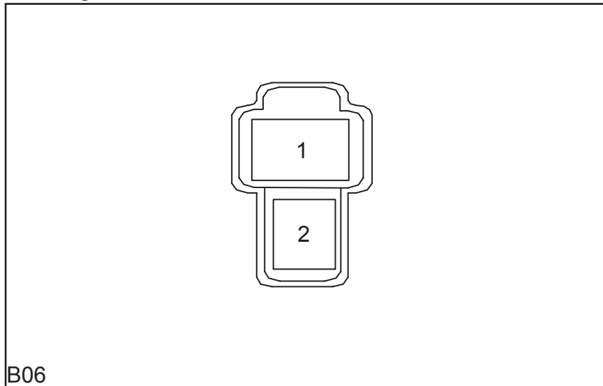
Passenger Side Seat Belt Switch Connector
