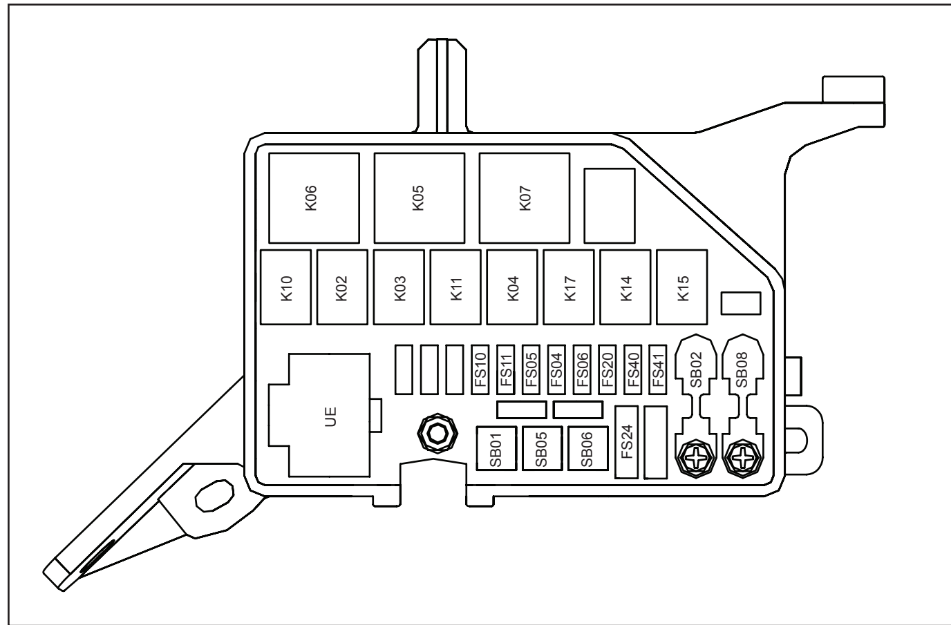
Engine Compartment Fuse and Relay Box
