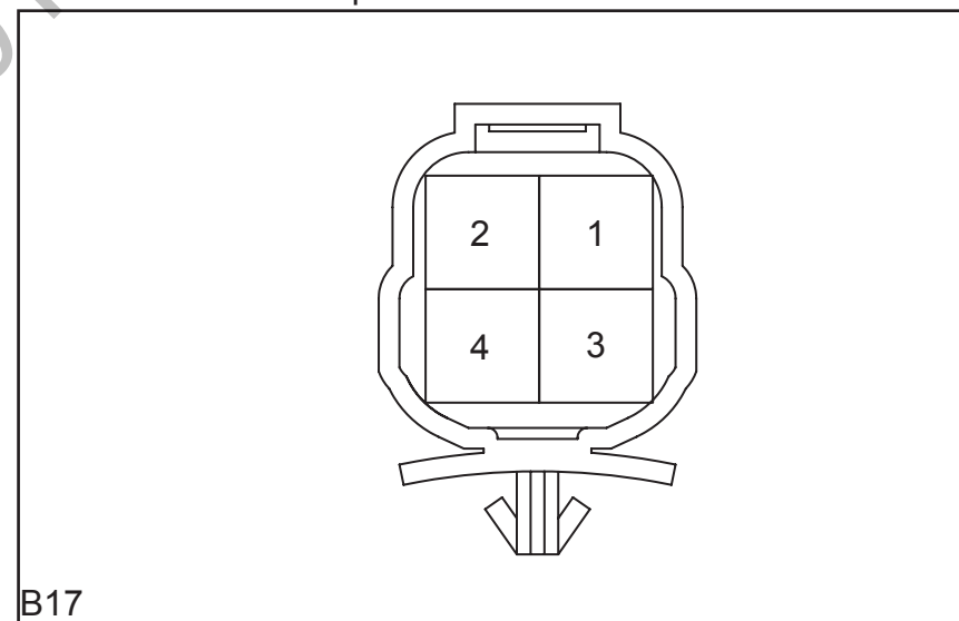
LR Combination Lamp Connector
