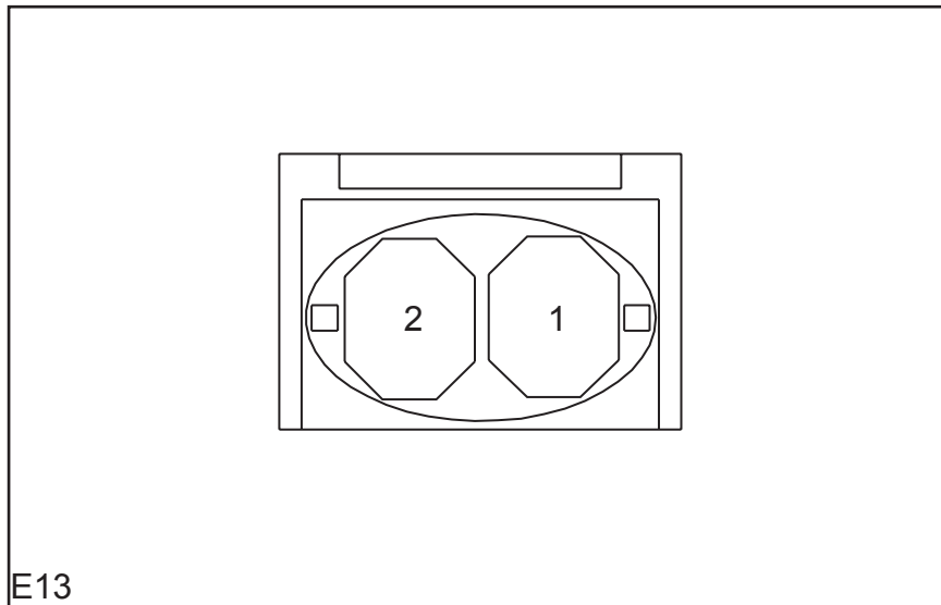
Knock Sensor Connector
