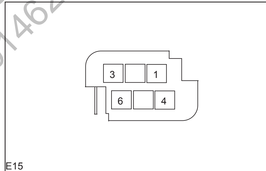
Electronic Throttle Valve Connector
