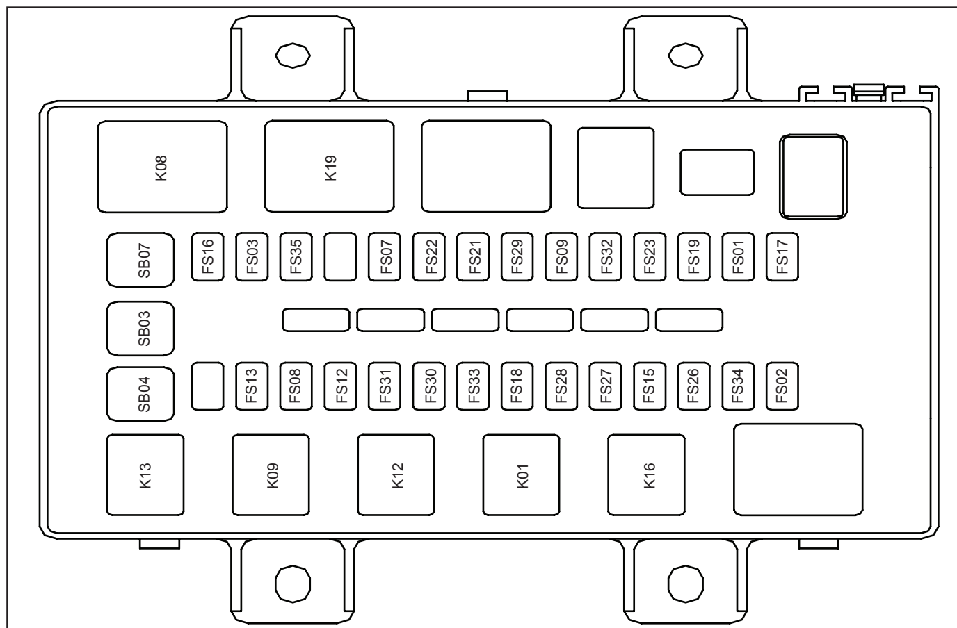
IP Fuse and Relay Box
