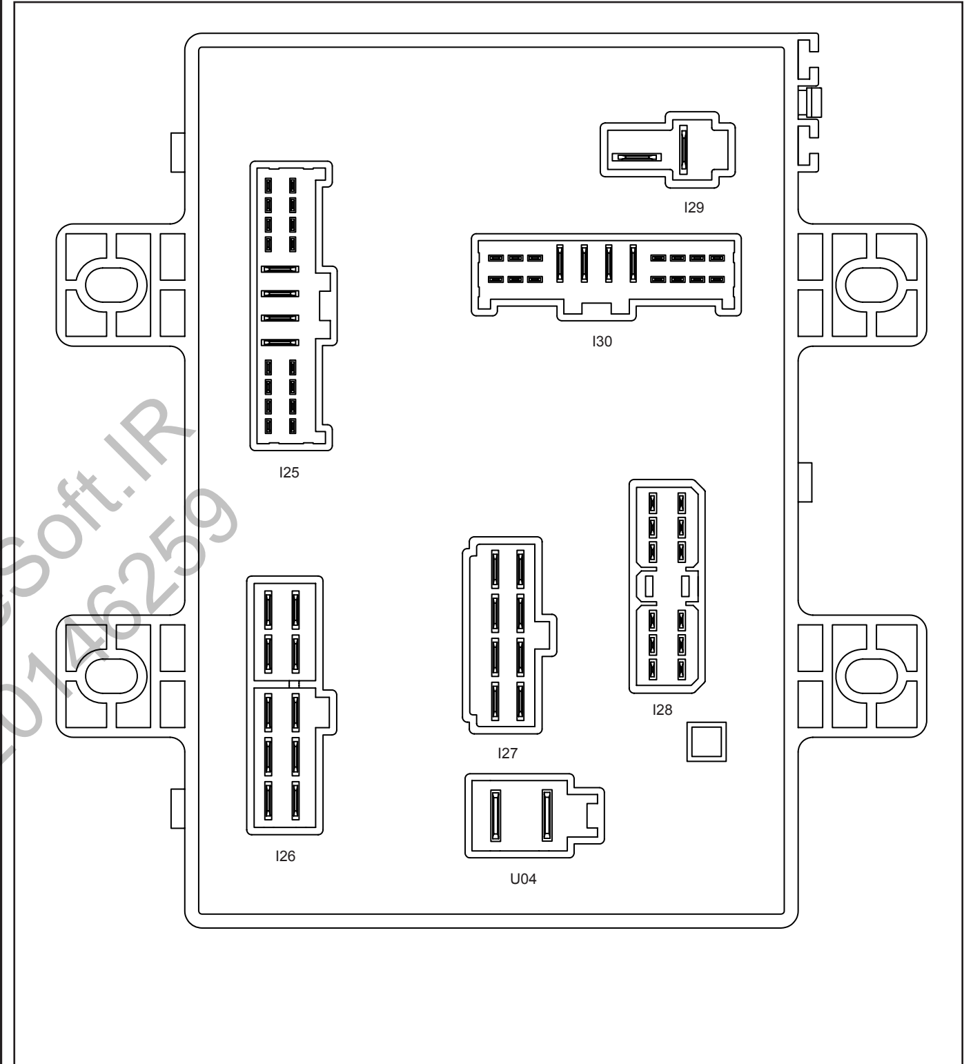
I/P Fuse and Relay Box Back View
