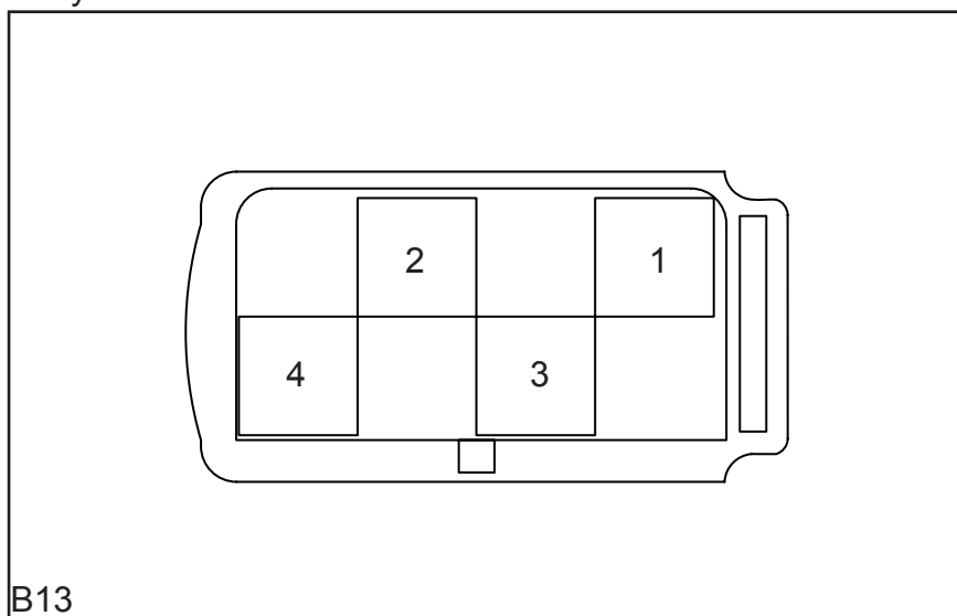
Body Harness Connector (B--) Body Yaw Rate Sensor Connector
