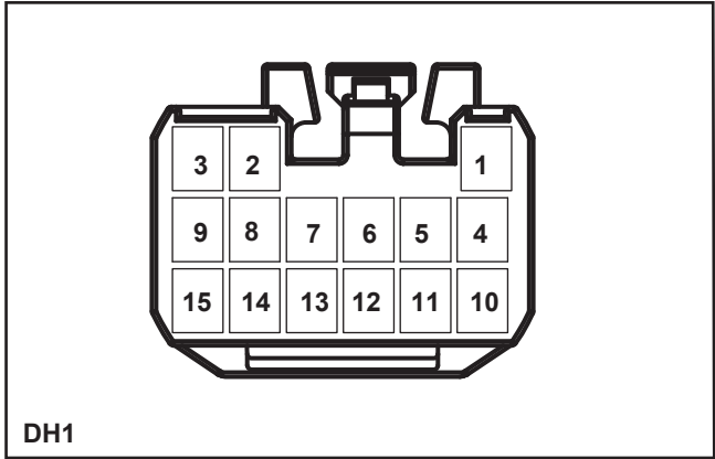
DH1 Pin Definition
