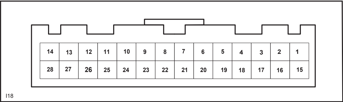
I18 Pin Definition
