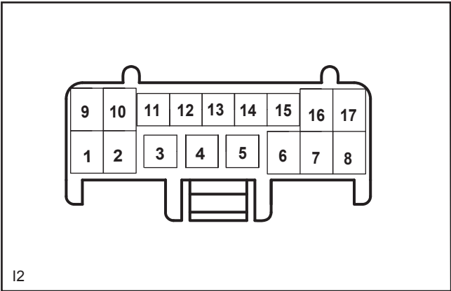
I2 Pin Definition
