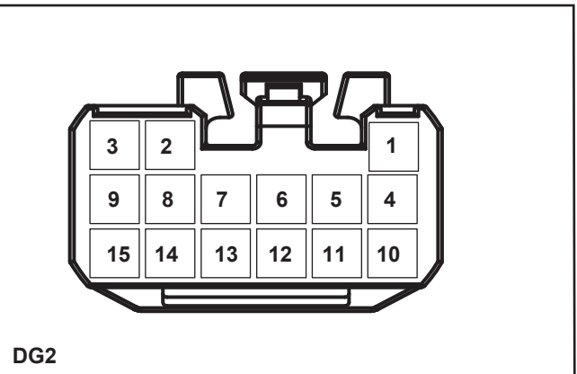
DG2 Pin Definition
