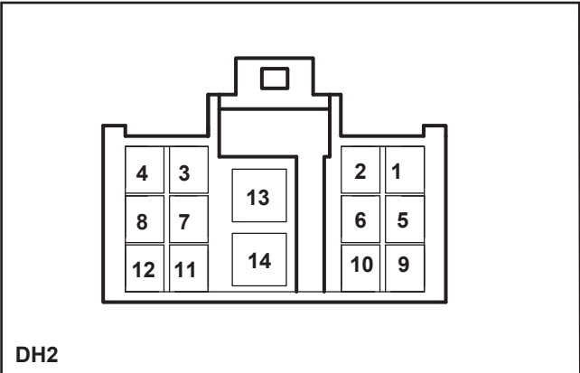
DH2 Pin Definition
