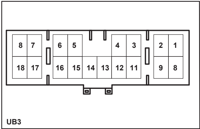
UB3 Pin Definition
