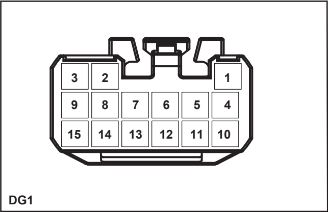
DG1 Pin Definition
