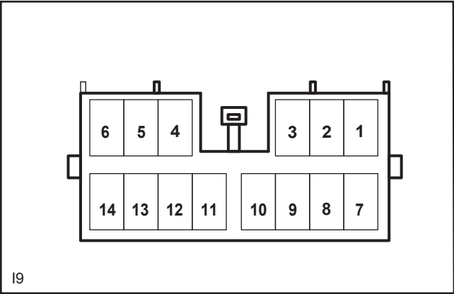
I9 Pin Definition
